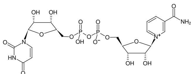
Structural formula of UP 2 (Nic)
