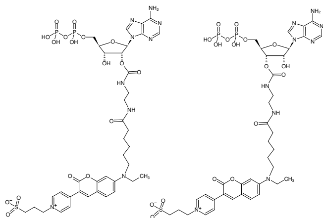
Structural formula of EDA-ADP-DY-485XL
