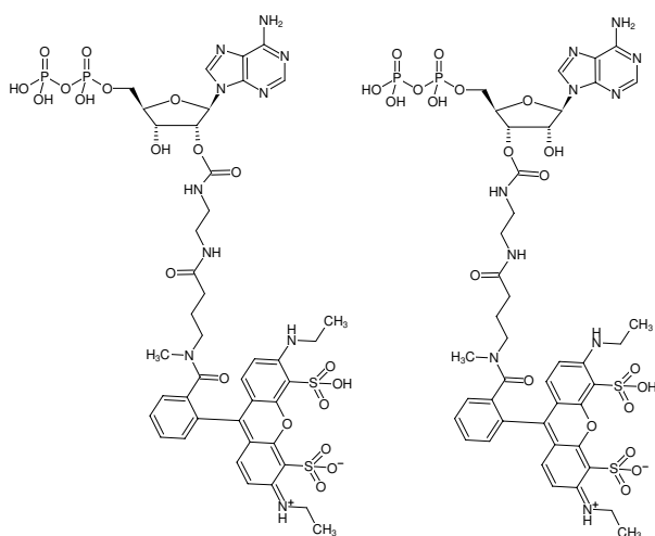
Structural formula of EDA-ADP-ATTO-532
