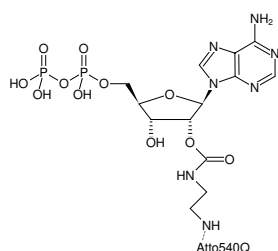
Structural formula of EDA-ADP-ATTO-540Q
