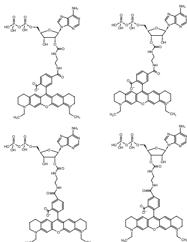
Structural formula of EDA-ADP-ATTO-565
