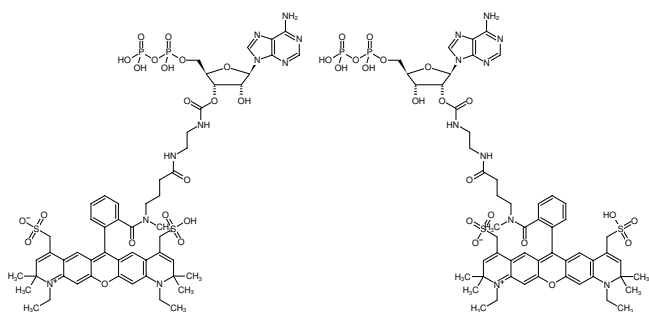
Structural formula of EDA-ADP-ATTO-594
