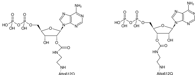
Structural formula of EDA-ADP-ATTO-612Q
