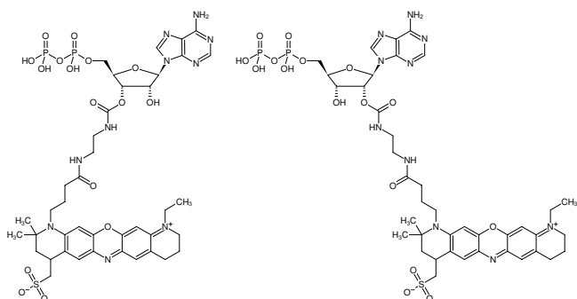
Structural formula of EDA-ADP-ATTO-655
