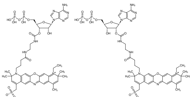
Structural formula of EDA-ADP-ATTO-700
