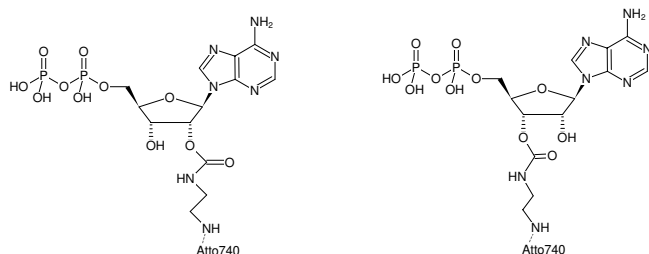
Structural formula of EDA-ADP-ATTO-740
