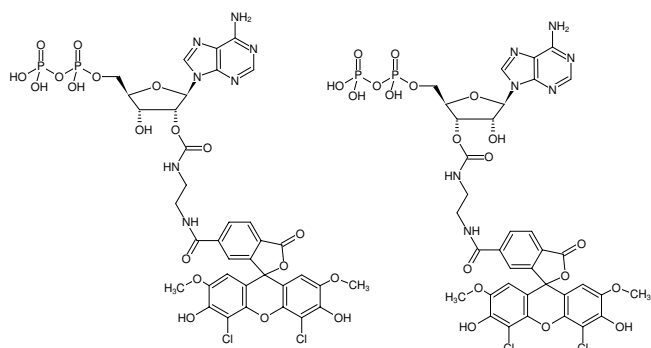
Structural formula of EDA-ADP-6-JOE
