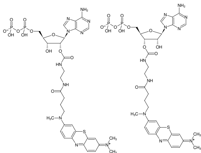
Structural formula of EDA-ADP-ATTO-MB2
