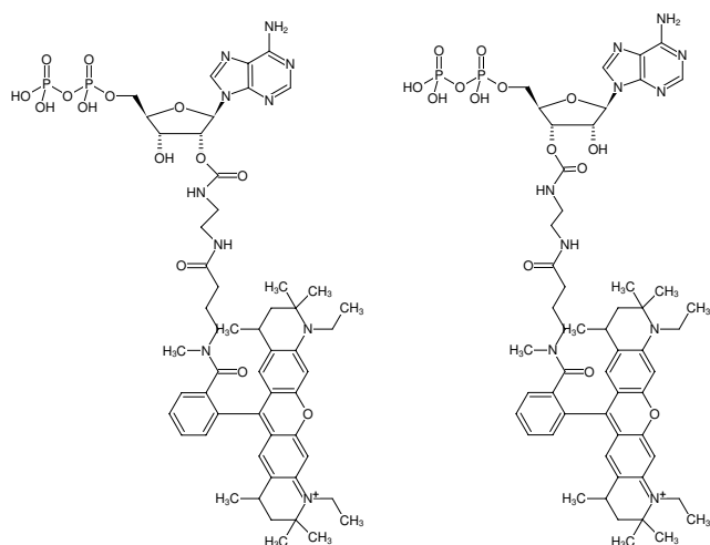
Structural formula of EDA-ADP-ATTO-Rho12
