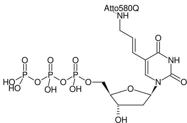
Structural formula of Aminoallyl-dUTP-ATTO-580Q
