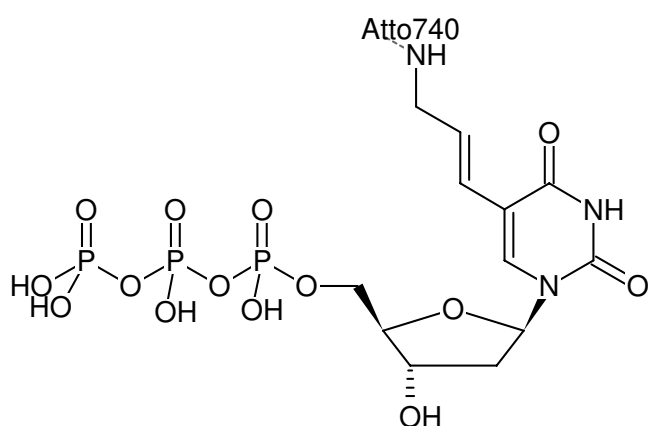
Structural formula of Aminoallyl-dUTP-ATTO-740
