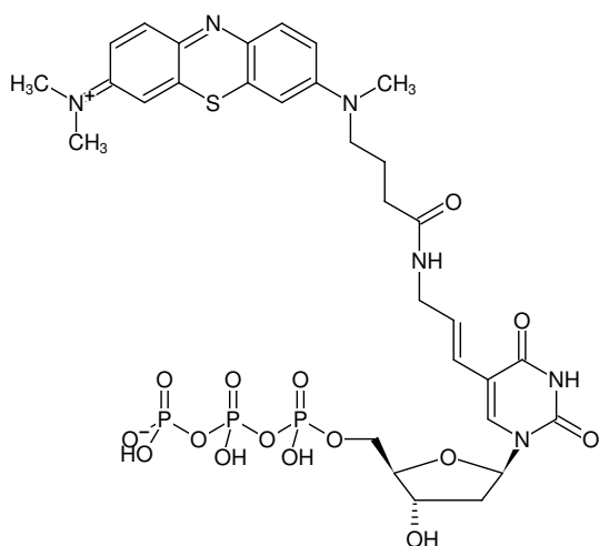
Structural formula of Aminoallyl-dUTP-ATTO-MB2
