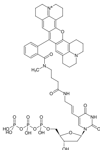
Structural formula of Aminoallyl-dUTP-ATTO-Rho101
