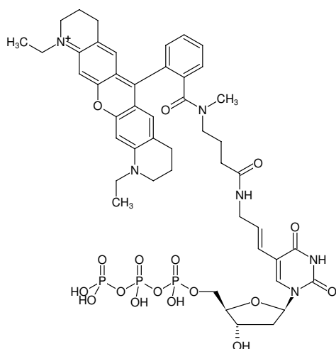
Structural formula of Aminoallyl-dUTP-ATTO-Rho11
