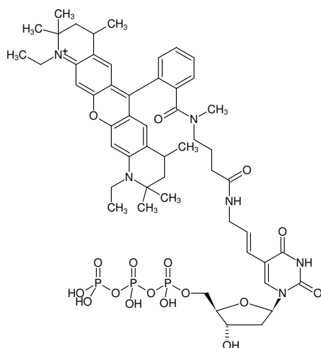
Structural formula of Aminoallyl-dUTP-ATTO-Rho12
