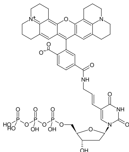
Structural formula of Aminoallyl-dUTP-6-ROX
