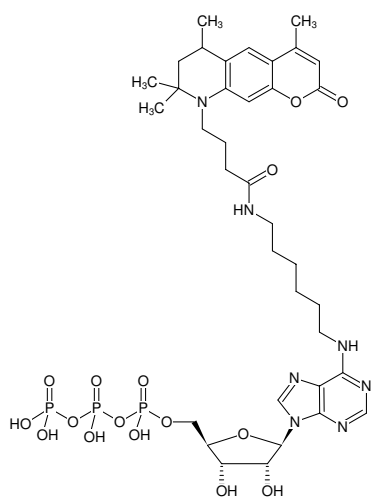
Structural formula of N 6 -(6-Aminoethyl)-ATP-ATTO-390
