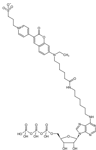
Structural formula of N 6 -(6-Aminoethyl)-ATP-DY-485XL
