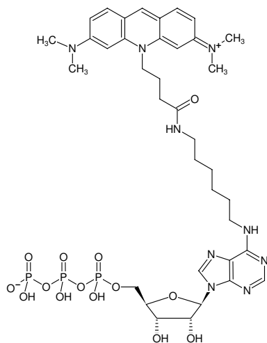
Structural formula of N 6 -(6-Aminoethyl)-ATP-ATTO-495
