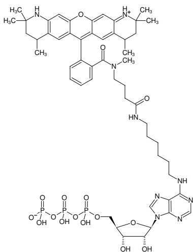
Structural formula of N 6 -(6-Aminoethyl)-ATP-ATTO-550
