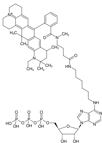
Structural formula of N 6 -(6-Aminoheptyl)-ATP-ATTO-647N
