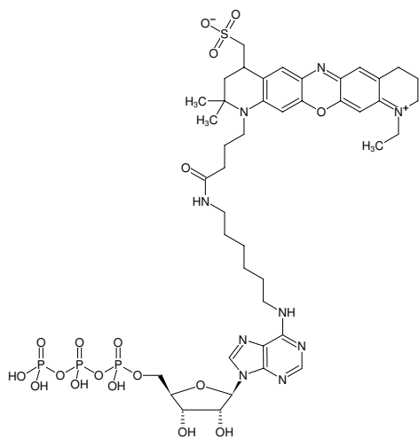
Structural formula of N 6 -(6-Aminoheptyl)-ATP-ATTO-655
