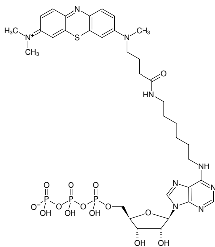
Structural formula of N 6 -(6-Aminoethyl)-ATP-ATTO-MB2
