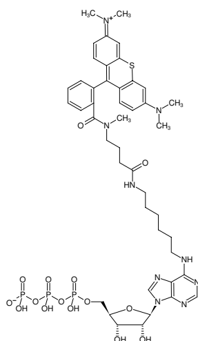
Structural formula of N 6 -(6-Aminoethyl)-ATP-ATTO-Thio12
