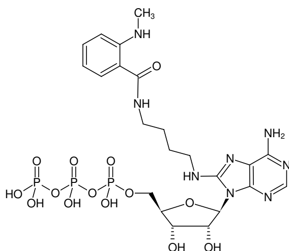
Structural formula of 8-[(4-Amino)butyl]-amino-ATP-MANT
