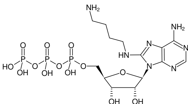
Structural formula of 8-[(4-Amino)butyl]-amino-ATP
