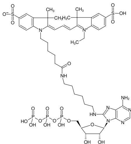
Structural formula of 8-(6-Aminoethyl)-amino-ATP-Cy3
