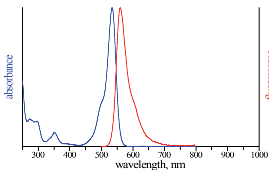
excitation and emission spectrum of ATTO Rho6G
