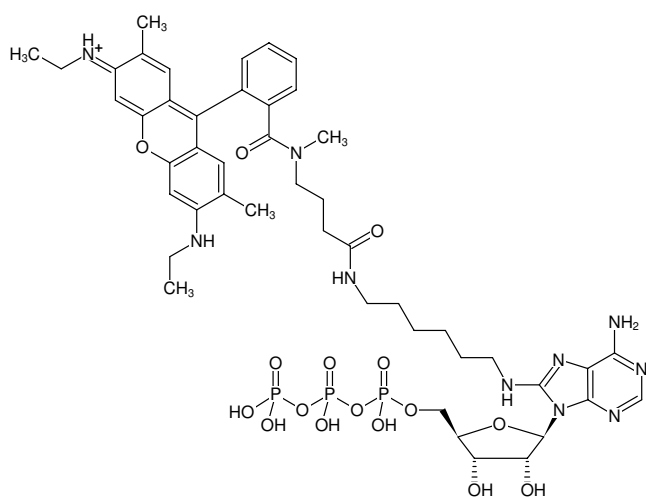
Structural formula of 8-(6-Aminoethyl)-amino-ATP-ATTO-Rho6G
