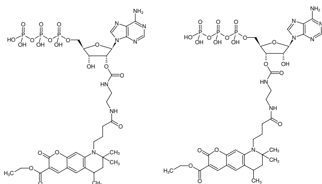
Structural formula of EDA-ATP-ATTO-425
