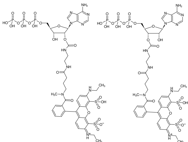
Structural formula of EDA-ATP-ATTO-532
