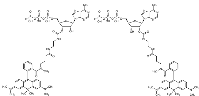
Structural formula of EDA-ATP-ATTO-620
