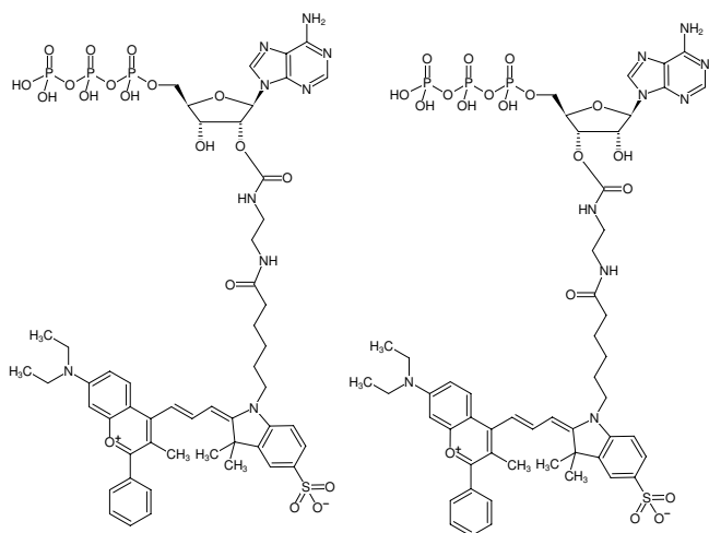
Structural formula of EDA-ATP-DYQ-660
