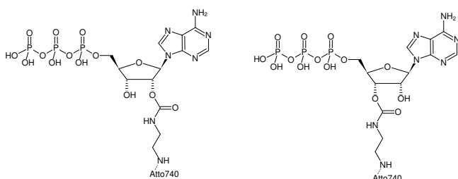
Structural formula of EDA-ATP-ATTO-740
