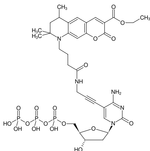
Structural formula of 5-Propargylamino-dCTP-ATTO-425
