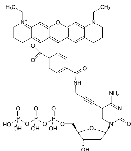
Structural formula of 5-Propargylamino-dCTP-ATTO-565
