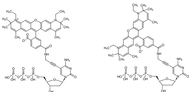
Structural formula of 5-Propargylamino-dCTP-ATTO-590
