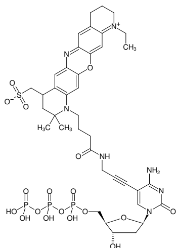
Structural formula of 5-Propargylamino-dCTP-ATTO-655
