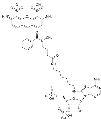
Structural formula of 8-(6-Aminoethyl)-amino-adenosine-3',5'-bisphosphate-ATTO-488
