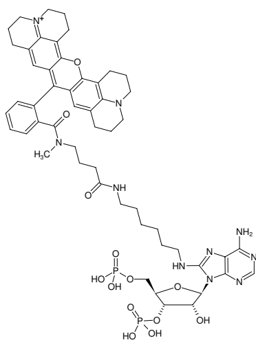
Structural formula of 8-(6-Aminoethyl)-amino-adenosine-3',5'-bisphosphate-ATTO-Rho101
