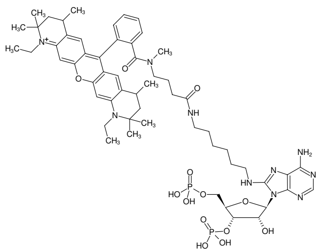
Structural formula of 8-(6-Aminoethyl)-amino-adenosine-3',5'-bisphosphate-ATTO-Rho12
