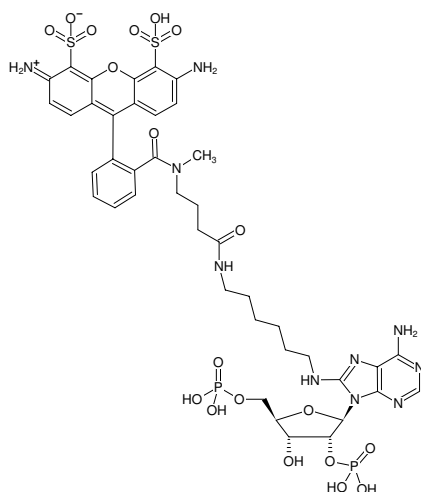
Structural formula of 8-(6-Aminoethyl)-amino-adenosine-2',5'-bisphosphate-ATTO-488
