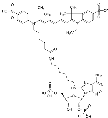
Structural formula of 8-(6-Aminoethyl)-amino-adenosine-2',5'-bisphosphate-Cy5
