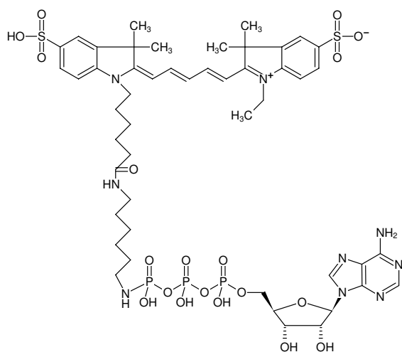
Structural formula of \gamma -[(6-Aminoethyl)-imido]-ATP-Cy5
