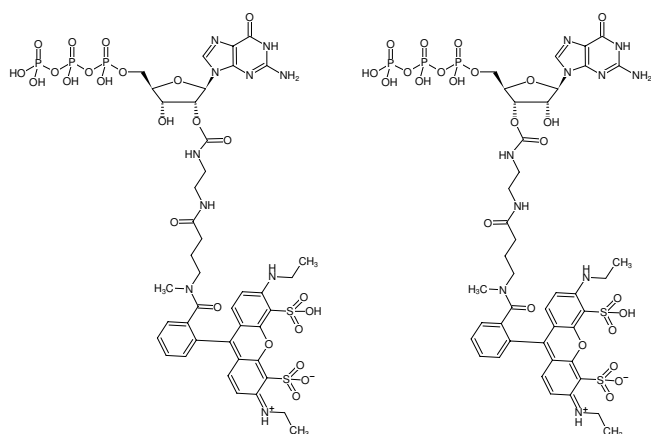
Structural formula of EDA-GTP-ATTO-532
