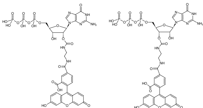
Structural formula of EDA-GTP-5-FAM
