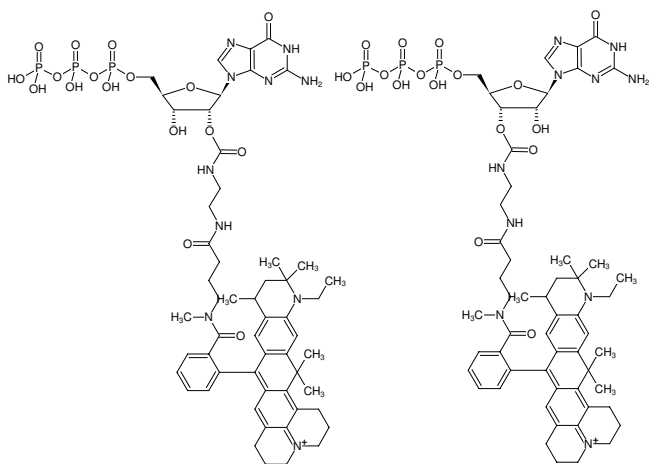
Structural formula of EDA-GTP-ATTO-647N
